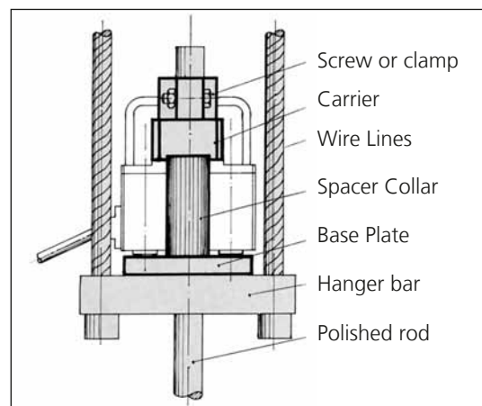
Installation of the spacers
