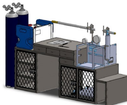
Customized PVT Sampling Container (interior view)
